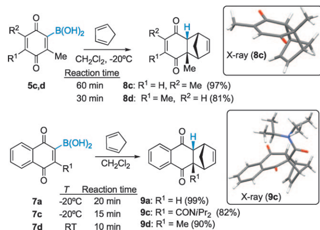
Scheme 3. Reactions of 5c and d and 7a , c and d with cyclopentadiene and X-ray structures of 8c and 9c .
