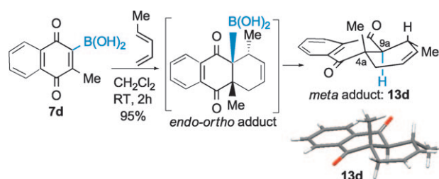
Scheme 7. Reaction of 7d with piperylene and X-ray structure of trans -fused 13d .
