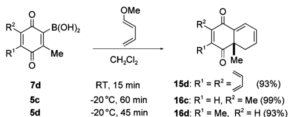
Scheme 9. Reactions of 7d , 5c and 5d with 1-methoxy-1,3-butadiene.
