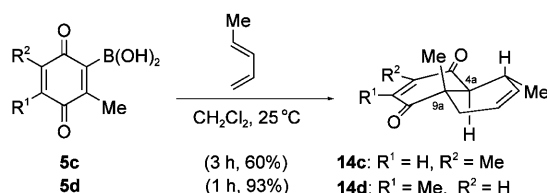
Scheme 8. Reactions of 5c and 5d with piperylene.
