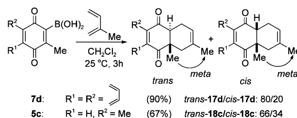
Scheme 10. Reactions of 3-methyl-2-quinonyl boronic acids 7d and 5c with isoprene.
