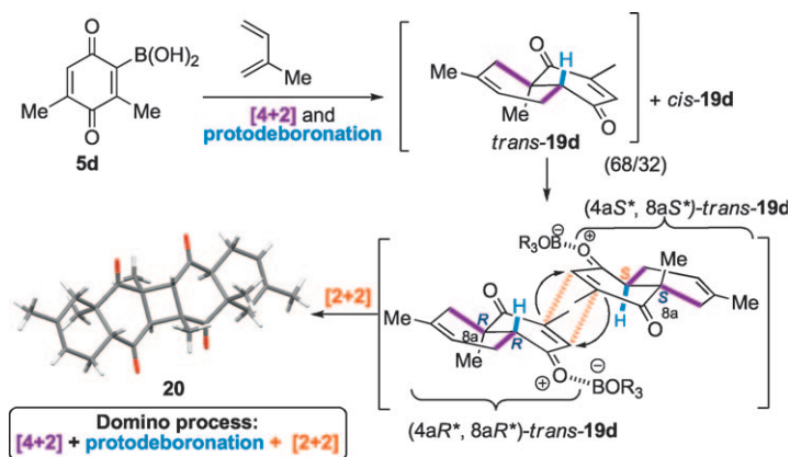
Scheme 16. Plausible formation and X-ray structure of dimer 20 .
