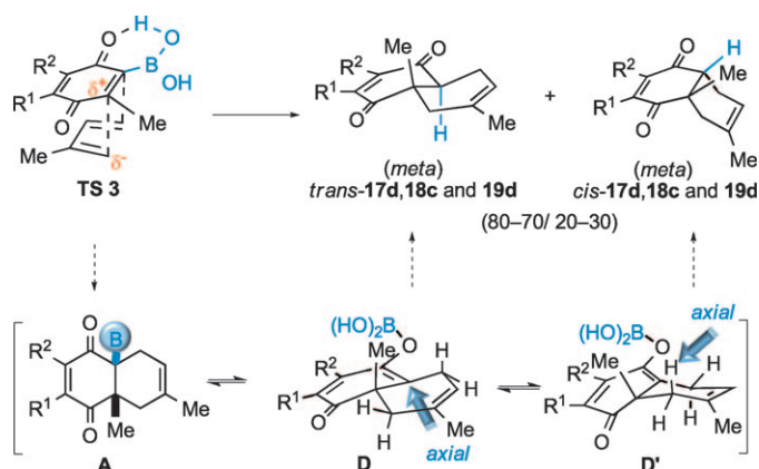
Scheme 15. Regio- and stereochemical course of the domino Diels-Alder reactions and protodeboronation of quinonyl boronic acids with piperylene.
