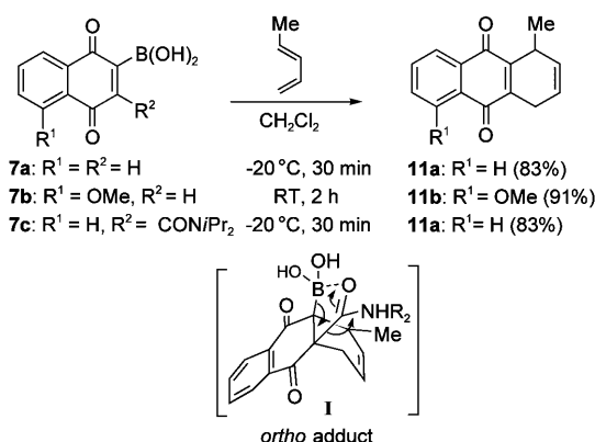
Scheme 5. Reactions of 2-naphthoquinonyl boronic acids 7a–c with piperylene.
