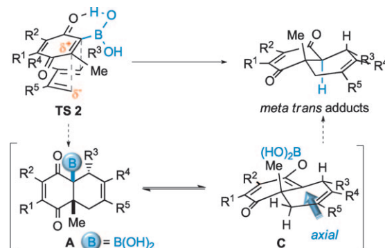
Scheme 14. Regio- and stereochemical course of the domino Diels-Alder reactions and protodeboronation of quinonyl boronic acids with 1-substituted acyclic dienes.
