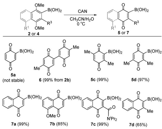
Scheme 2. Synthesis of 2-benzo and 2-naphthoquinonyl boronic acids 5 and 7 .
