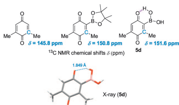
Figure 1. ^{13}\text{C} NMR chemical shifts of selected carbon atoms and X-ray structure of 5d .
