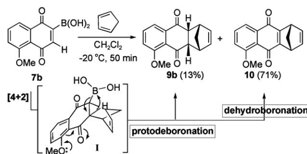
Scheme 4. Reaction of 7b with cyclopentadiene.
