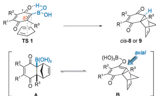
Scheme 13. Regio- and stereochemical course of the domino Diels-Alder reactions and protodeboronation of quinonyl boronic acids 5c-d , 7a , 7c and 7d with cyclopentadiene.
