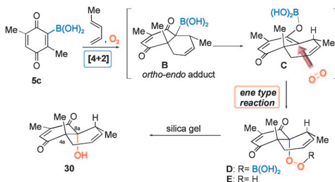
Scheme 17. Mechanistic proposal to justify the formation of hydroxy derivative 30 .
