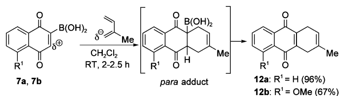
Scheme 6. Reactions of 2-naphthoquinonyl boronic acids 7a and b with isoprene.
