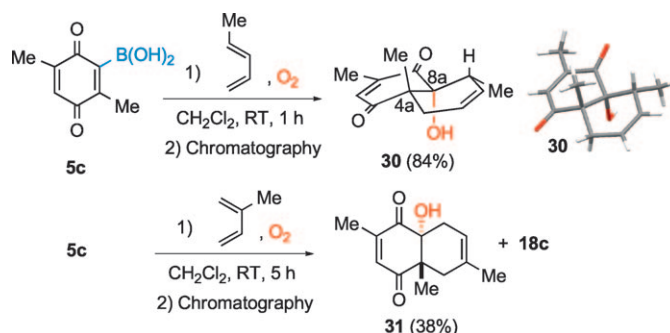
Scheme 12. Reactions of 5c with piperylene or isoprene under an oxygen atmosphere and X-ray structure of 30 .
