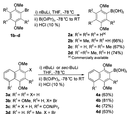
Scheme 1. Synthesis of phenyl boronic acids 2b–d and naphthyl boronic acids 4a–d .
