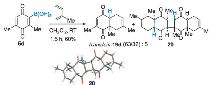
Scheme 11. Reaction of dimethylquinonyl boronic acid 5d with isoprene and X-ray structure of dimer 20 .
